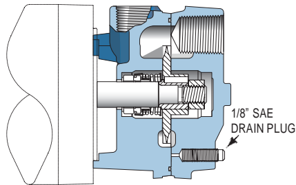
C15 Motor Frame
